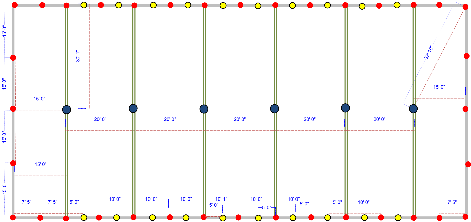
30' x 130' Pole Tent Standard & Wind - Pole Placements
